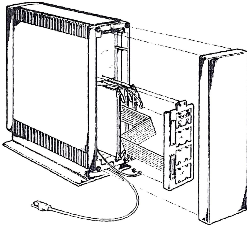
Figure 5-7 KFQSA Installation In a BA23 Enclosure
