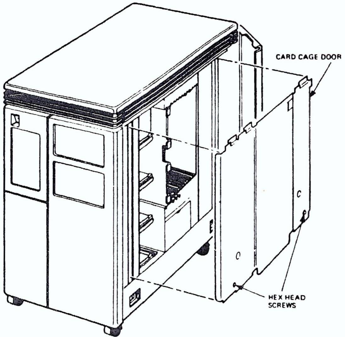
Figure 5-6 Removing the Card Cage Door
