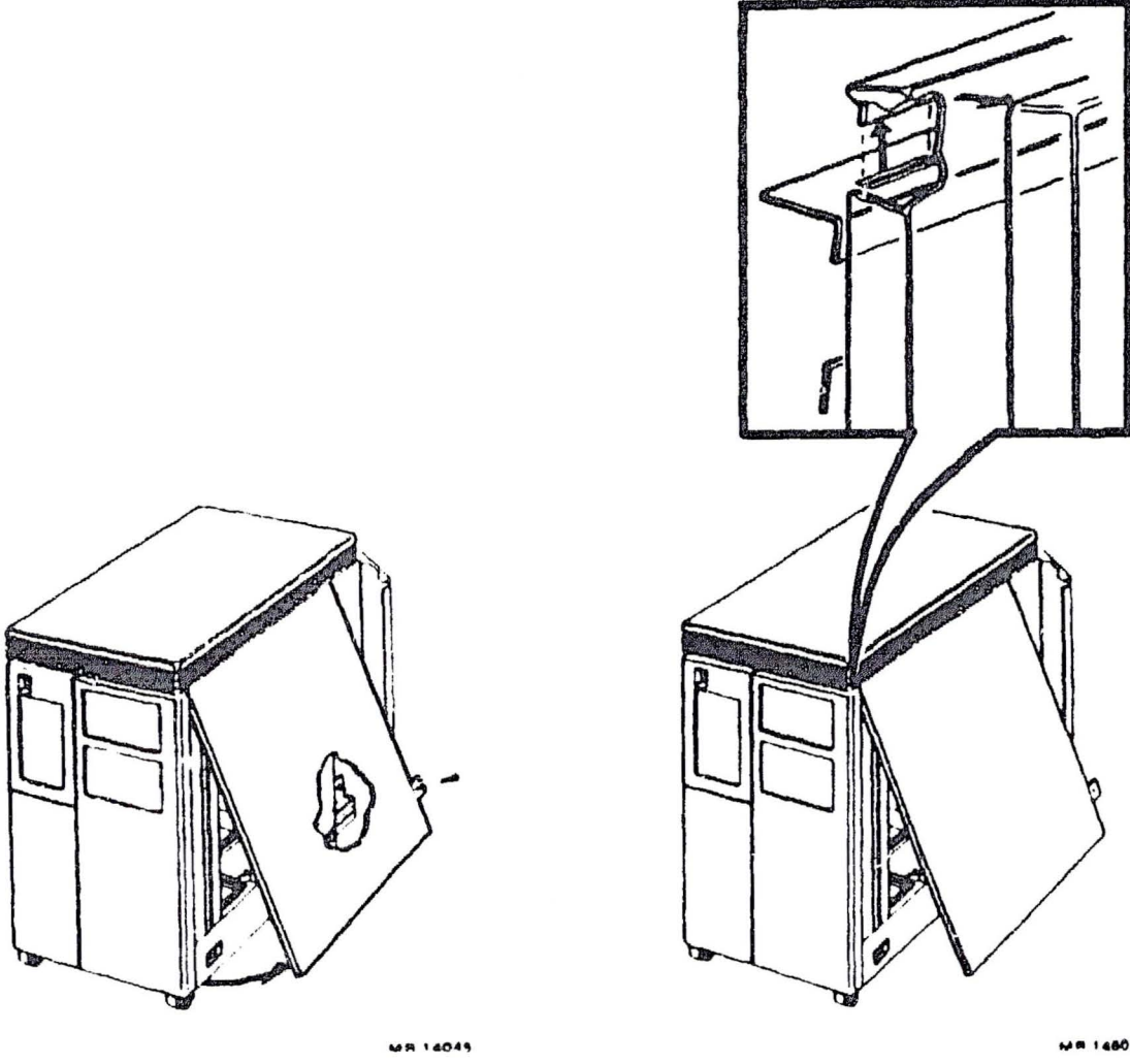
Figure 5-5 Removing the Right Side Panel
