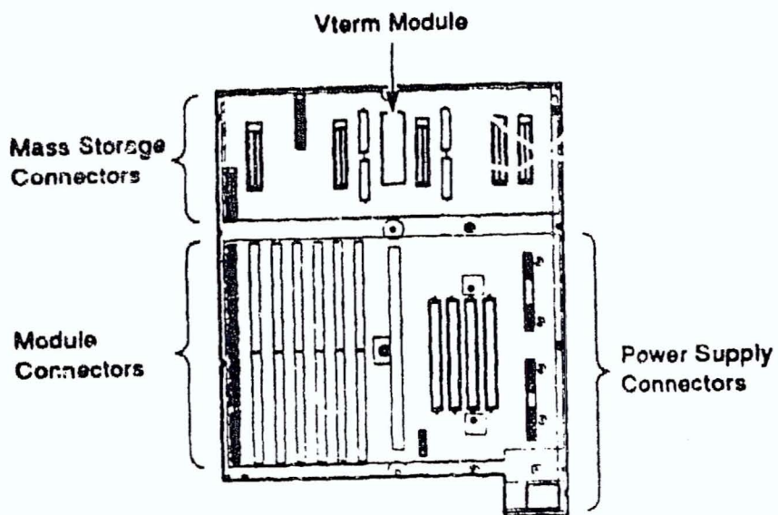
Figure 1-5 BA440 Backplane
