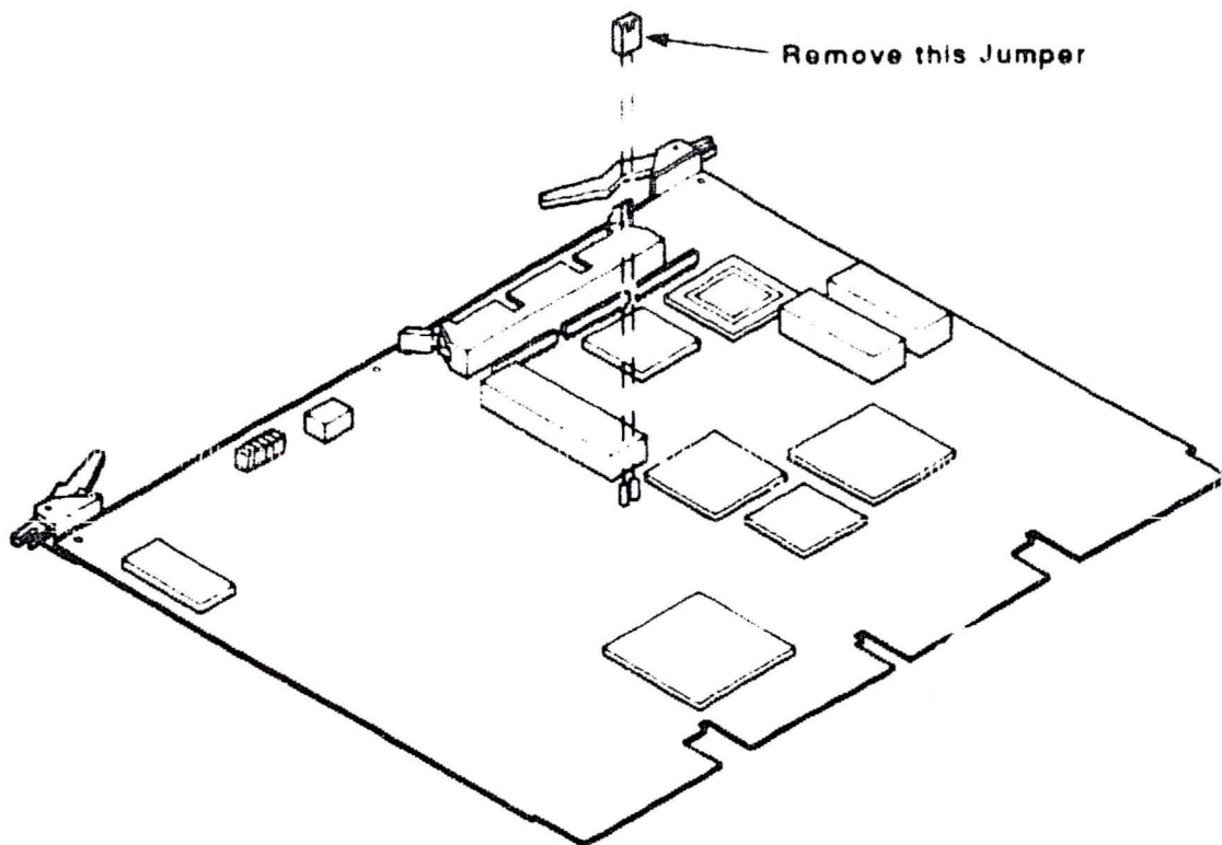
Figure 2-1 KFQSA Jumper Location
